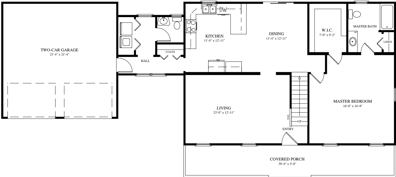
1st Floor Plan 8'-0" Ceiling
