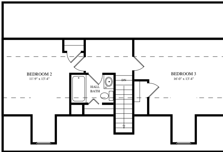
2nd Floor Plan 8'-0" Ceiling
