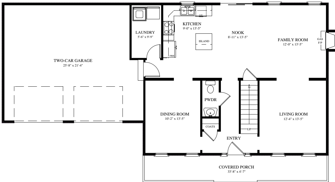
1st Floor Plan 8'-0" Ceiling
