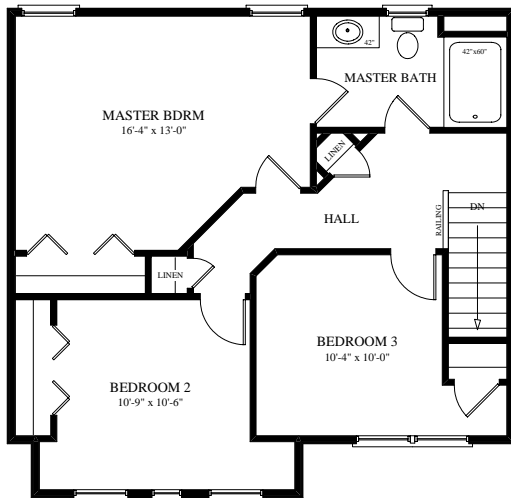
2nd Floor Plan 8'-0" Ceiling
